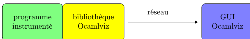
Figure 1 – Architecture d'Ocamlviz.
