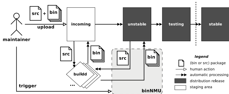
Figure 2: package (auto-)building in Debian.
